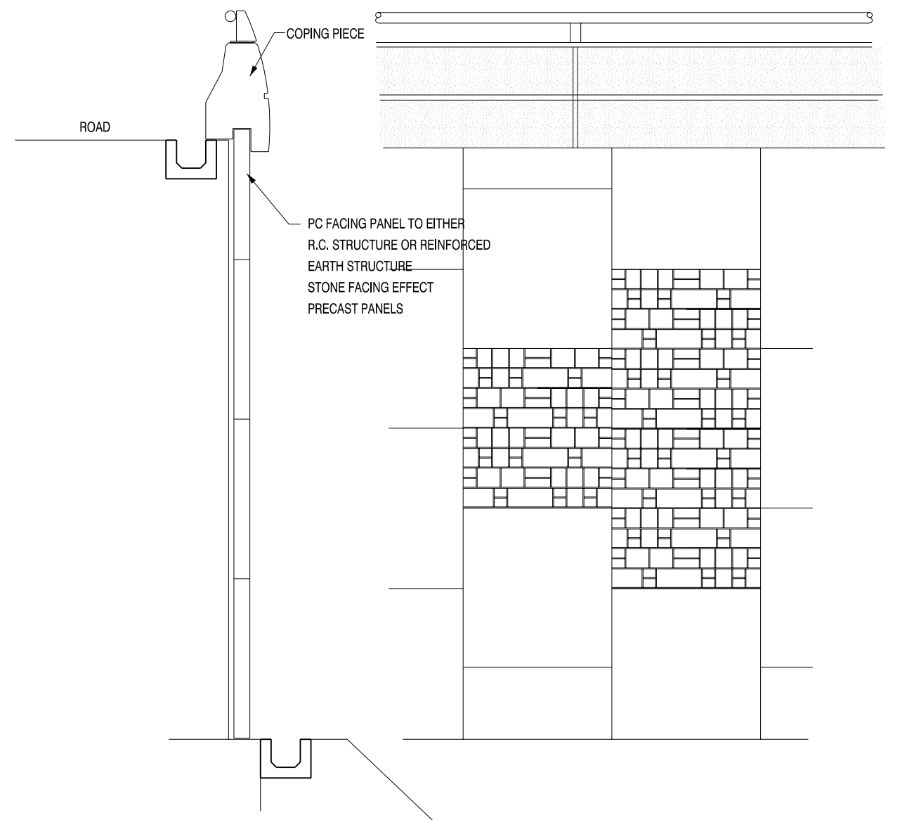
RETAINING WALL BELOW THE ROAD
