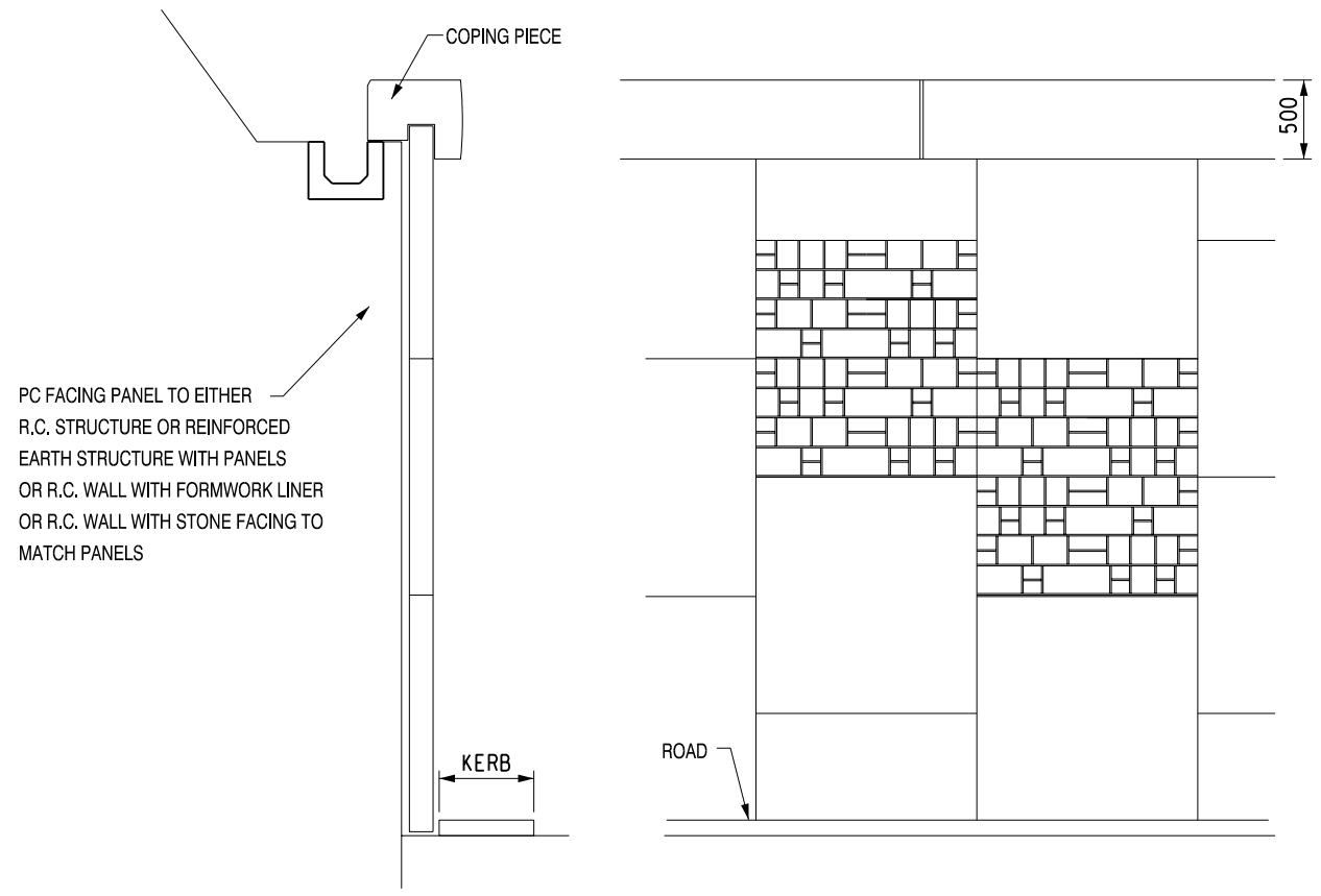
RETAINING WALL ABOVE THE ROAD
